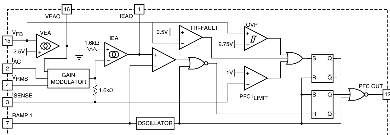
Figure 1. PFC Block Diagram
